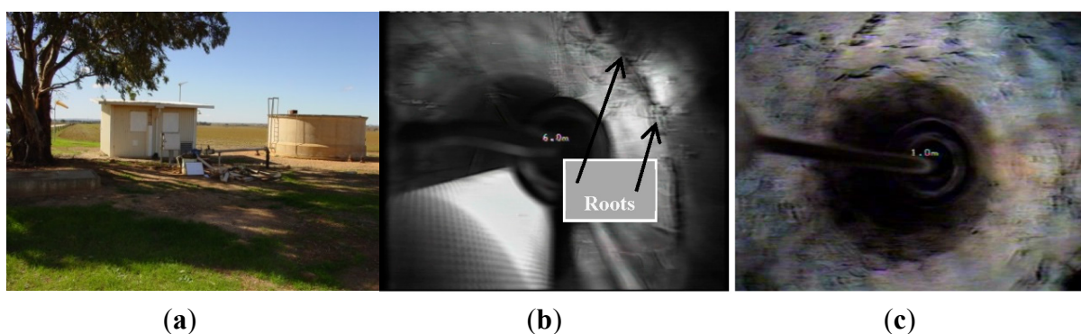
Figure 5. Failed well casings—pathways for contaminants; (a) tree in the vicinity of Melrose TWS 5; (b) roots penetration through opening between PVC casing joints-Melrose TWS 5; (c) steel casing corrosion and lamination in Lincoln basin.
